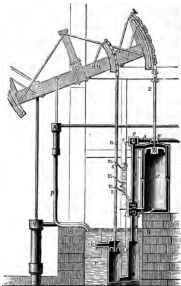
FIG. 26.—Watt's Engine, 1774.
